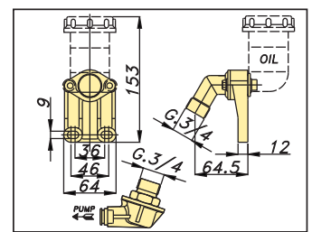
Serbatoio olio a distanza - Remote mounted oil tank - Выносной масляный бак
